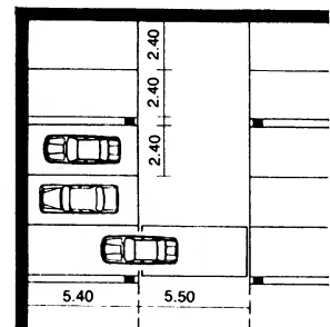
⑧ Cars moved on pallets (Wöhr system)
